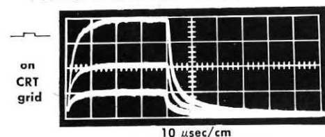
PHOSPHOR RISE and DECAY TIME
