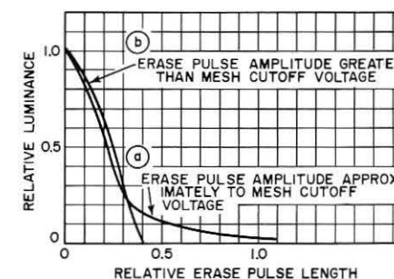
FIGURE 7: Typical DST erase characteristic.
