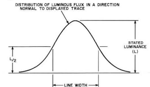
FIGURE 2: Definition of line width as used in the paper.
