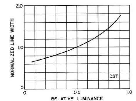
FIGURE 3: Line-width change as a function of luminance.
